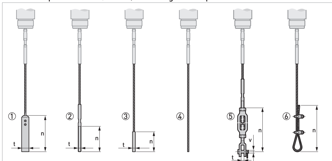
Figure 2-18: Probe end options for the Ø4 mm / 0.16" single cable probe
