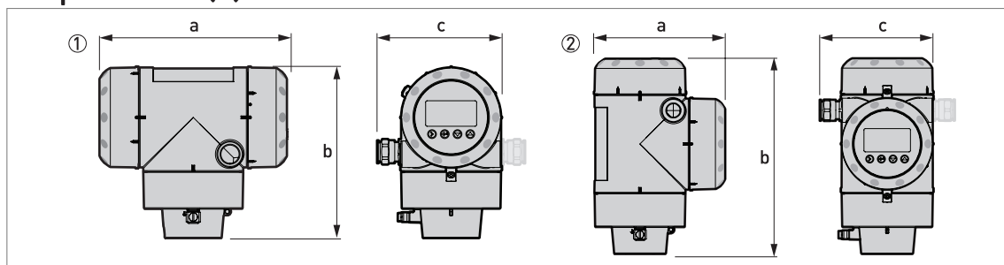
Figure 2-10: Compact version (C)
