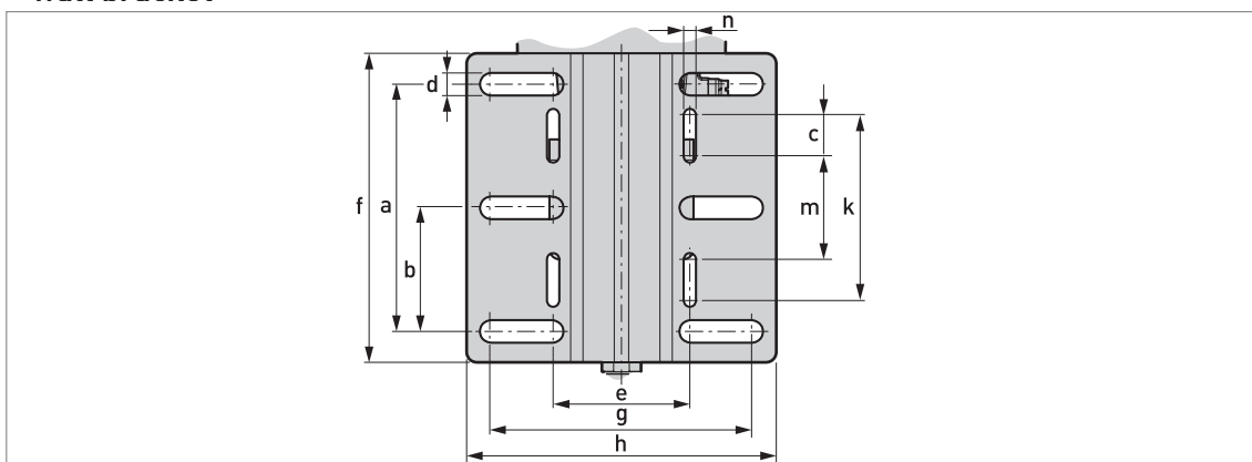
Figure 2-13: Wall bracket
